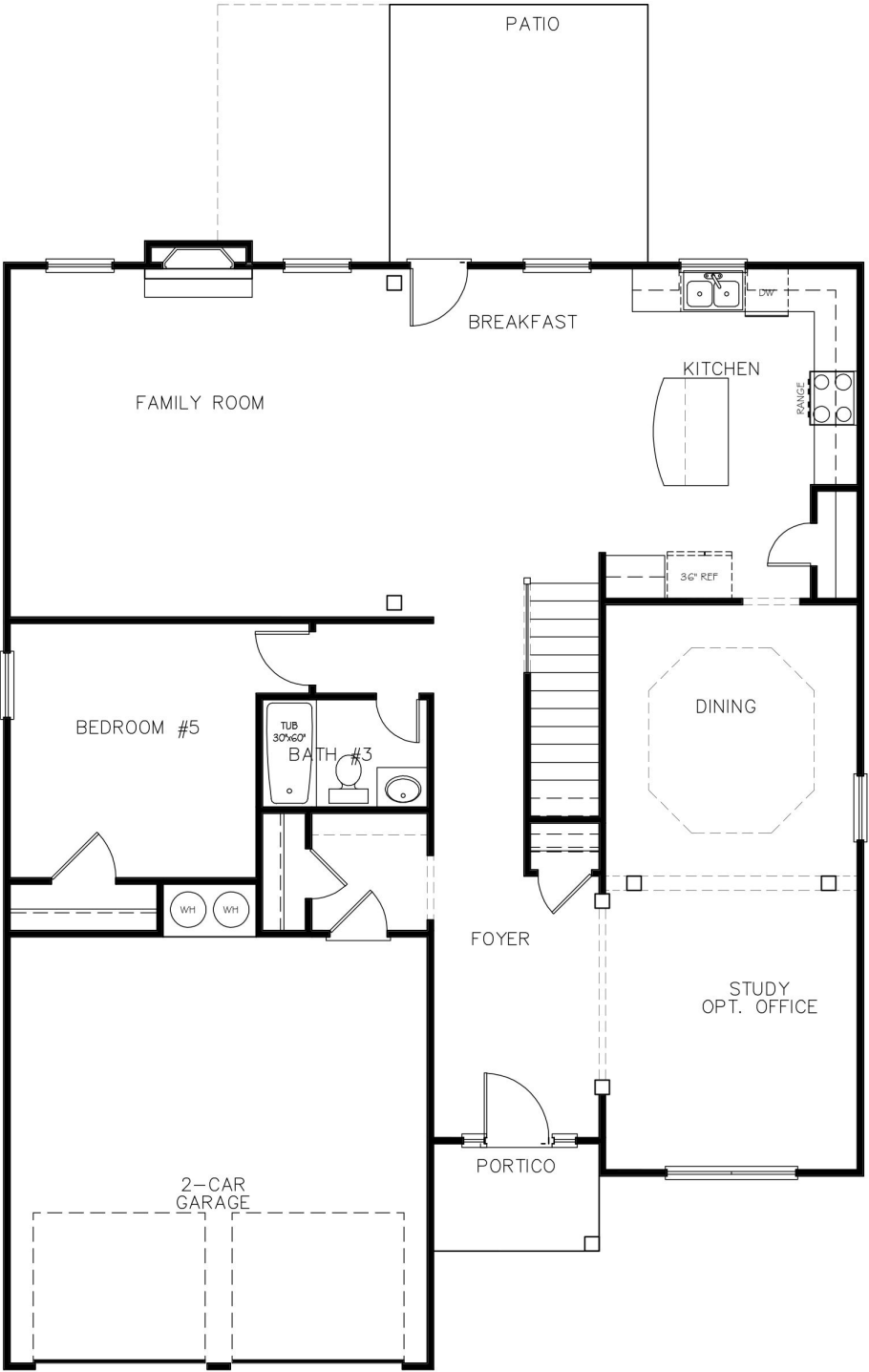
FIRST FLOOR
