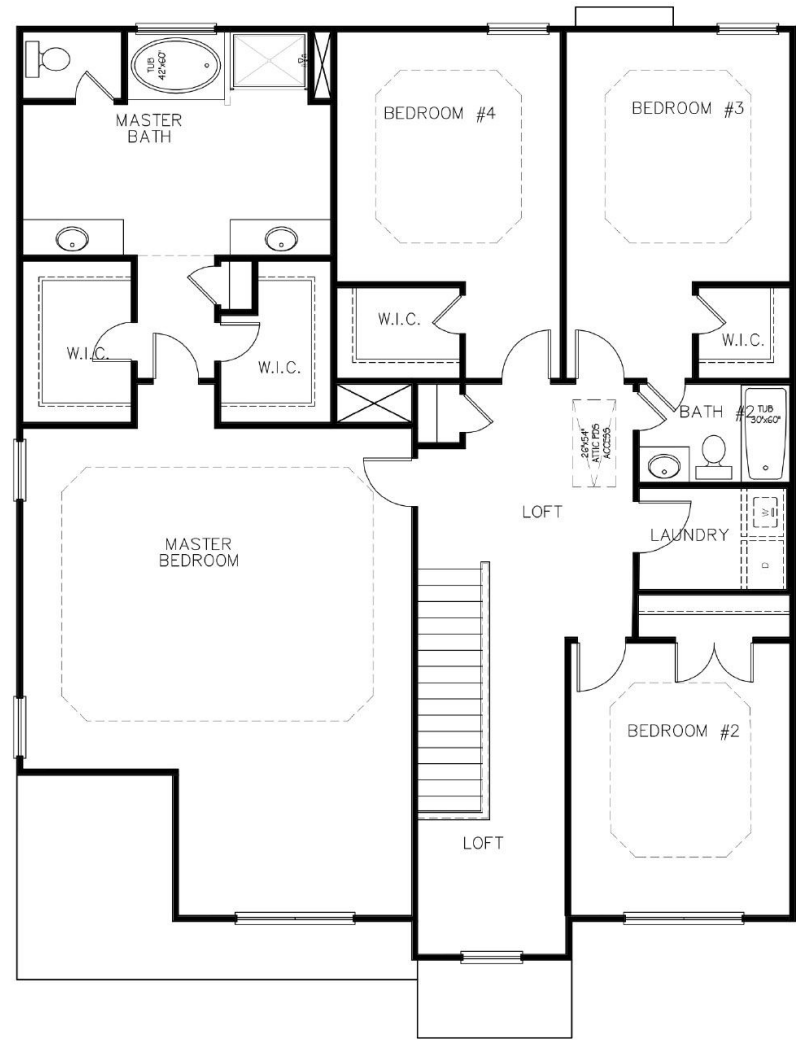
SECOND FLOOR
