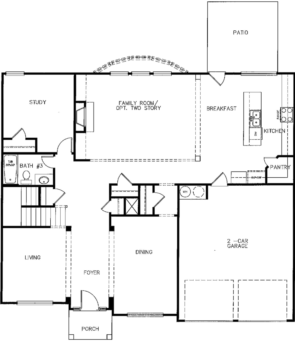
FIRST FLOOR
