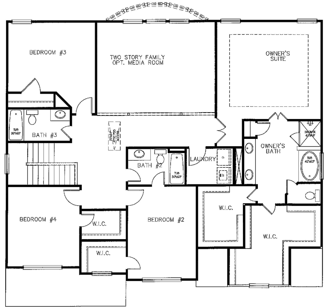
SECOND FLOOR
